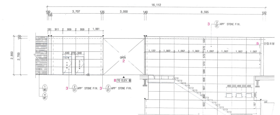
2층 접견실 입면 S' / 2nd floor reception area elevation S'
