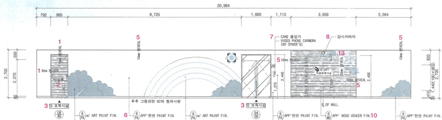
2층 어린이집 입면 V / 2nd floor children's room elevation V
