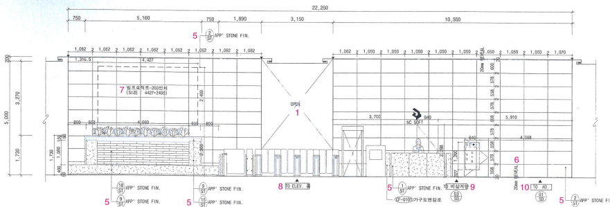
1층 로비 입면 Q / 1st floor lobby elevation Q
