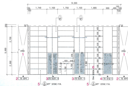
1층 엘리베이터 홀 입면 P / 1st floor elevator hall elevation P
