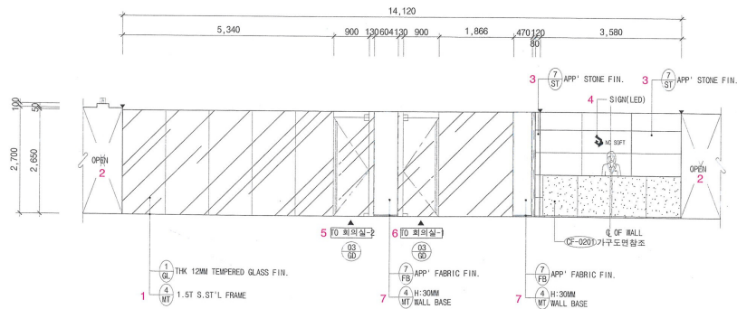
2층 접견실 입면 S / 2nd floor reception area elevation S
