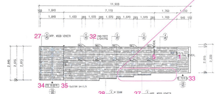
13층 다회의실 입면 Z / 13th floor multi-conference room elevation Z
