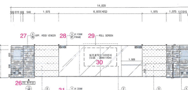
13층 다회의실 입면 Z / 13th floor multi-conference room elevation Z
