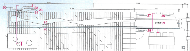
2층 접견실 연못 평면 / 2nd floor reception area pond plan
