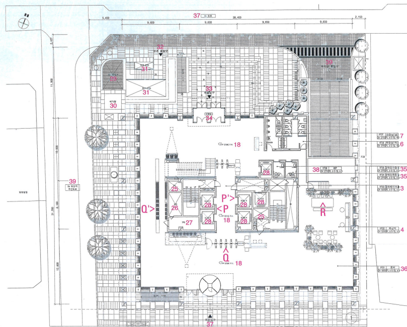
1층 평면도 / 1st floor plan
