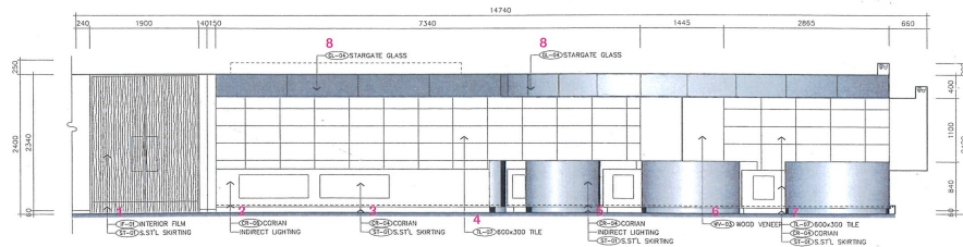
부페 입면 D / buffet restaurant elevation D
