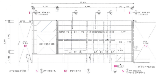
1층 로비 입면 Q' / 1st floor lobby elevation Q'
