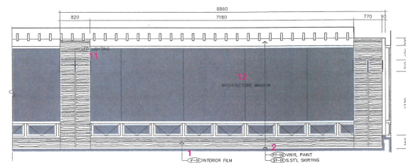
부페 입면 F' / buffet restaurant elevation F'
